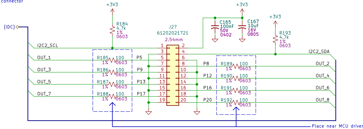
Valve connector
