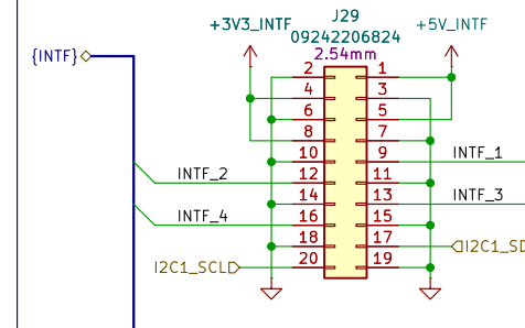
Backplane interface connector
